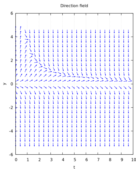
Figure 5.65: The direction field for y' = y(3 - ty) ( SymIntegration/Examples/Test SymIntegration Compute Direction Fields Part b/main.cpp ).
